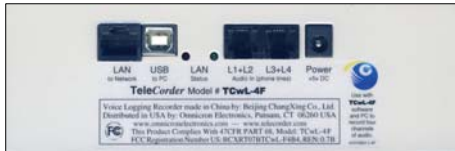
Back with input and output connections
